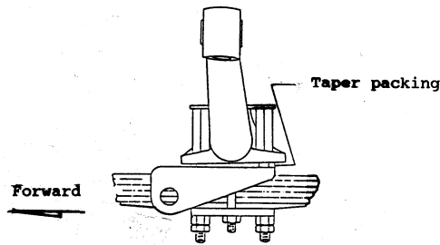
Figure 8 – Taper packing to change caster angle
