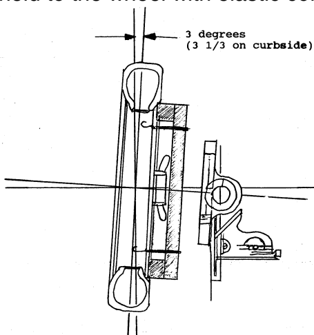
Figure 11 – Simple measuring device
