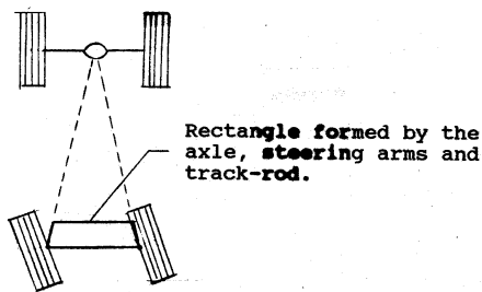
Figure 10 – Ackerman steering principle
