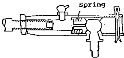
Figure 3 – Track rod assembly
