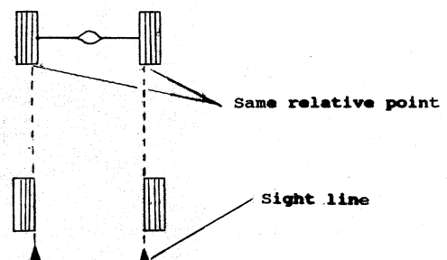
Figure 12 – Sighting front wheels
