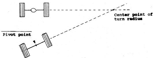
Figure 9 – Single pivot turning radius
