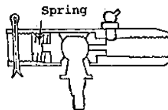
Figure 2 – Drop arm assembly
