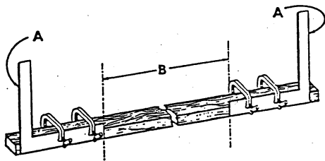
Figure 14 – Toe-in measuring device
