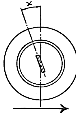
Figure 7 – Caster angle
