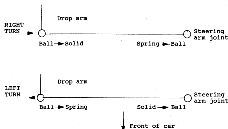
Figure 4 – Transmission of forces
