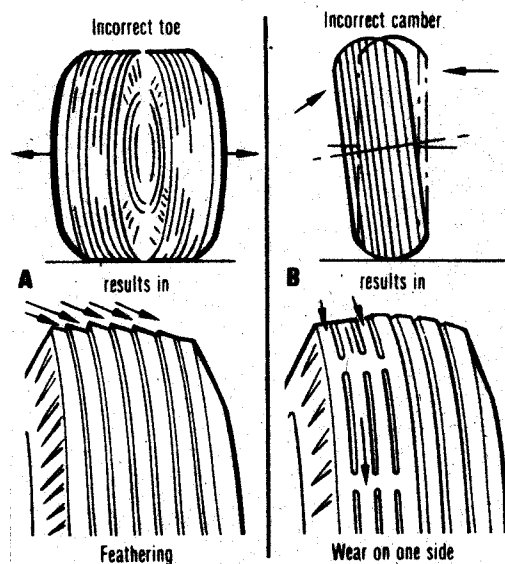
Figure 1 – Effects of incorrect set-up
