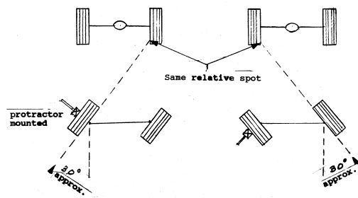
Figure 13 – Sight lines for measurement
