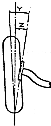
Figure 6 – Camber angle
