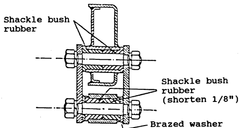
Figure 5 – Front spring, rear shackle
